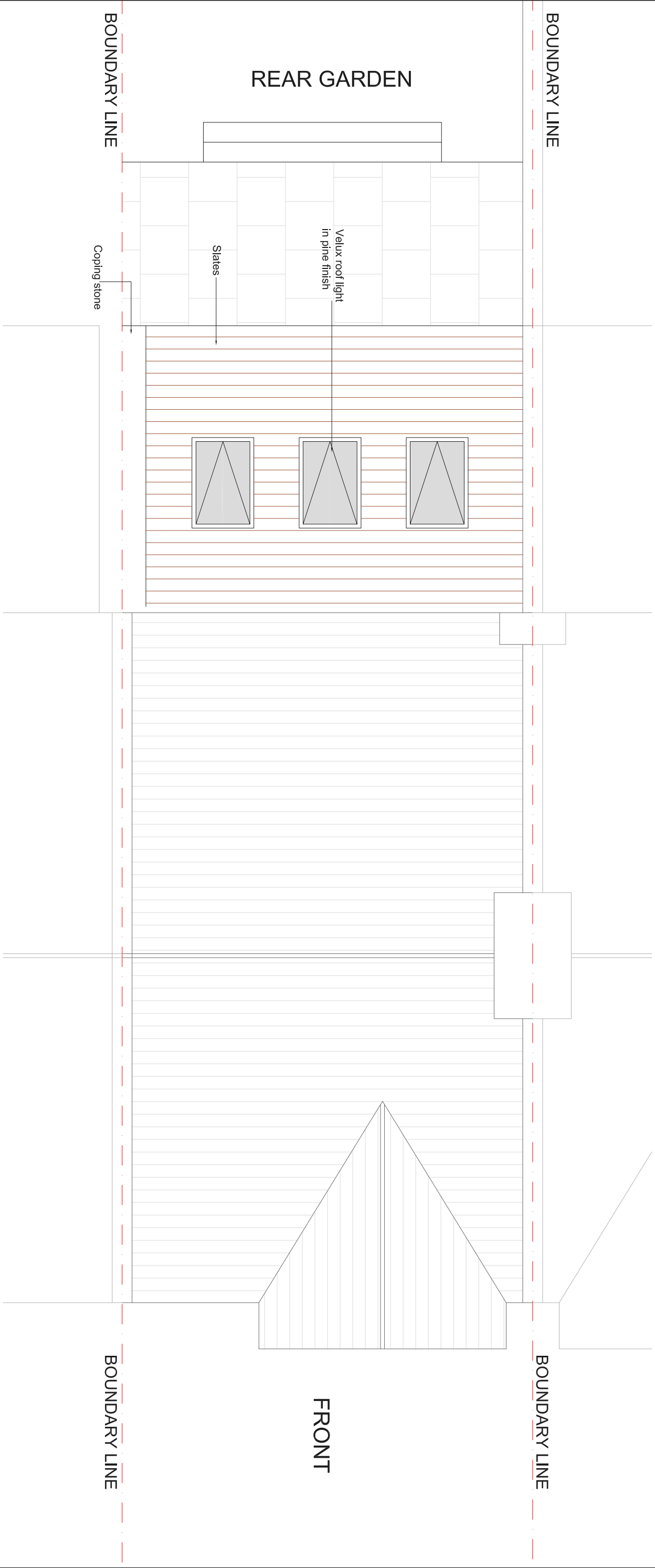
PROPOSED ROOF TOP PLAN SCALE 1:50
