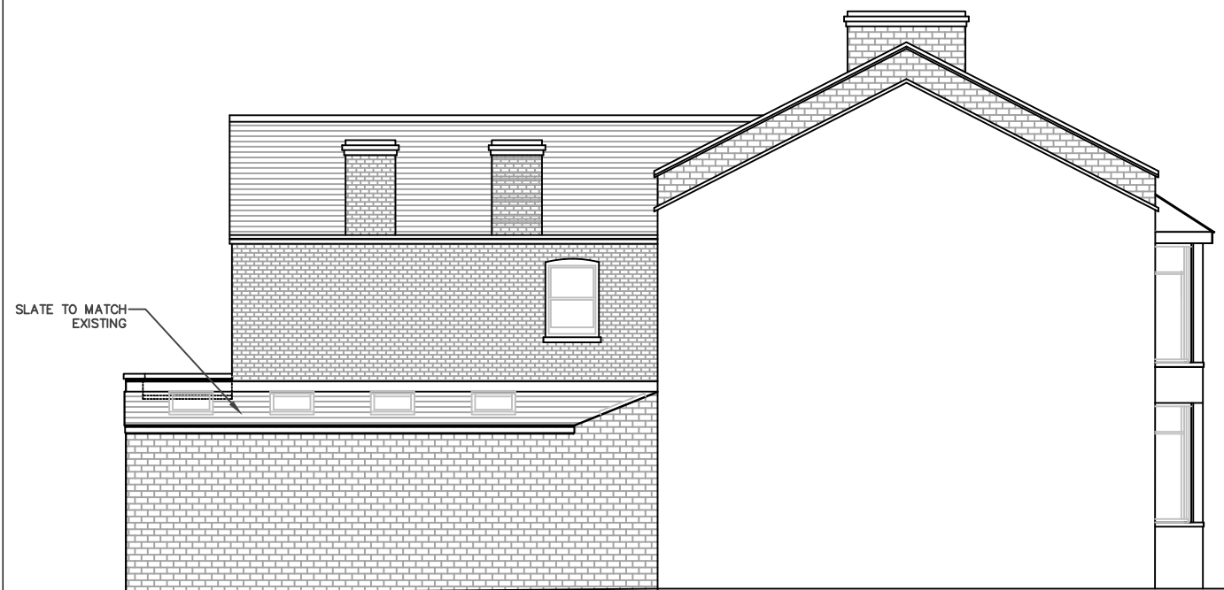
PROPOSED SIDE ELEVATION 1:50
